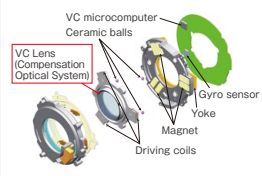
<Expanded VC Schematic Diagram>
